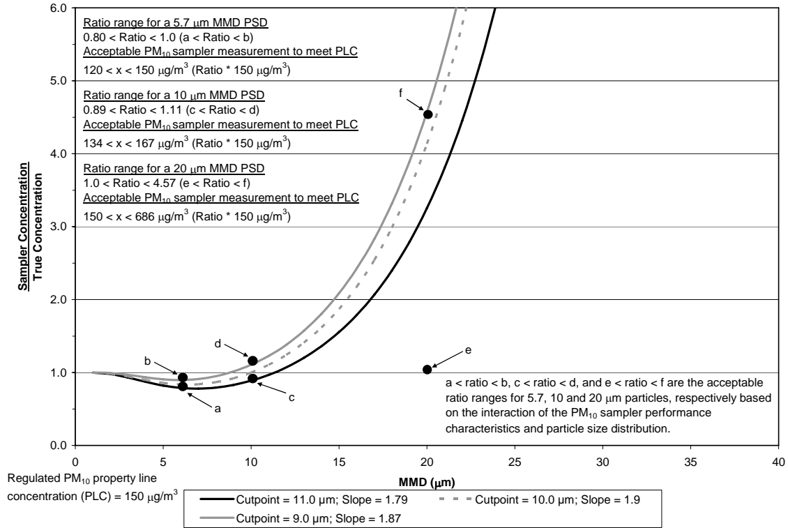
Figure 5. Theoretical ratios of \text{PM}_{10} stack sampler to true PSD concentrations (PSD – GSD = 1.5).
